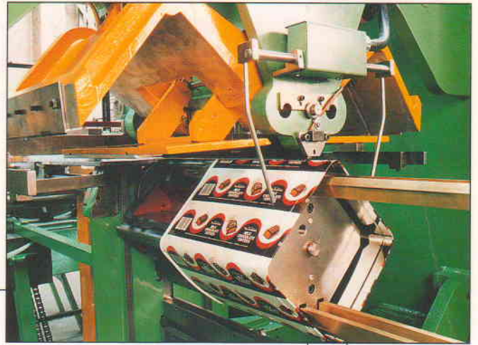
▲ Typical tooling for 613, showing expanded mandrel, forming wings and hammer blade.
