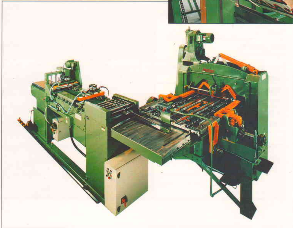
▲ Fully automatic 613 with beading and notching attachments.
